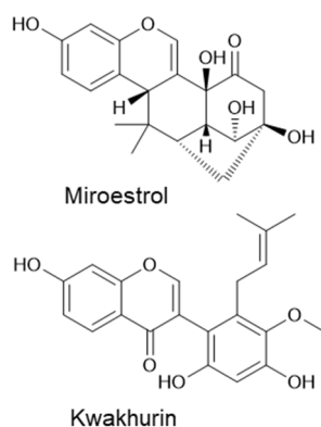
Fig. 1 Structures of miroestrol and kwakhurin
