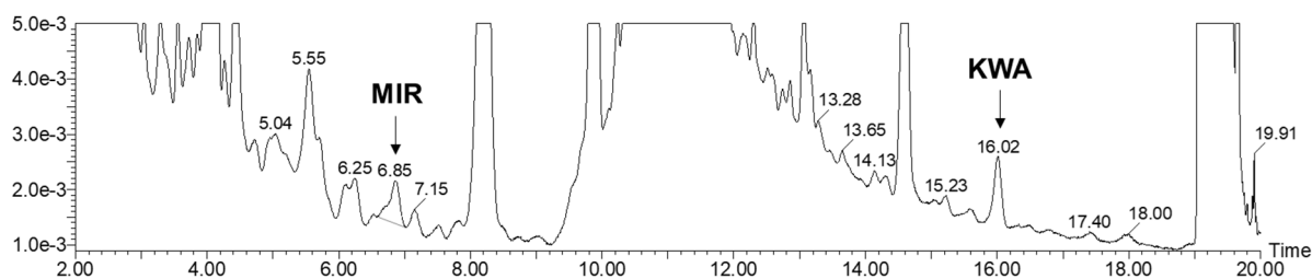
Fig. 2 Representative chromatogram of P. mirifica crude drug (PMC-1)
